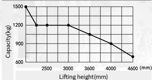
CAPACITY CHART
